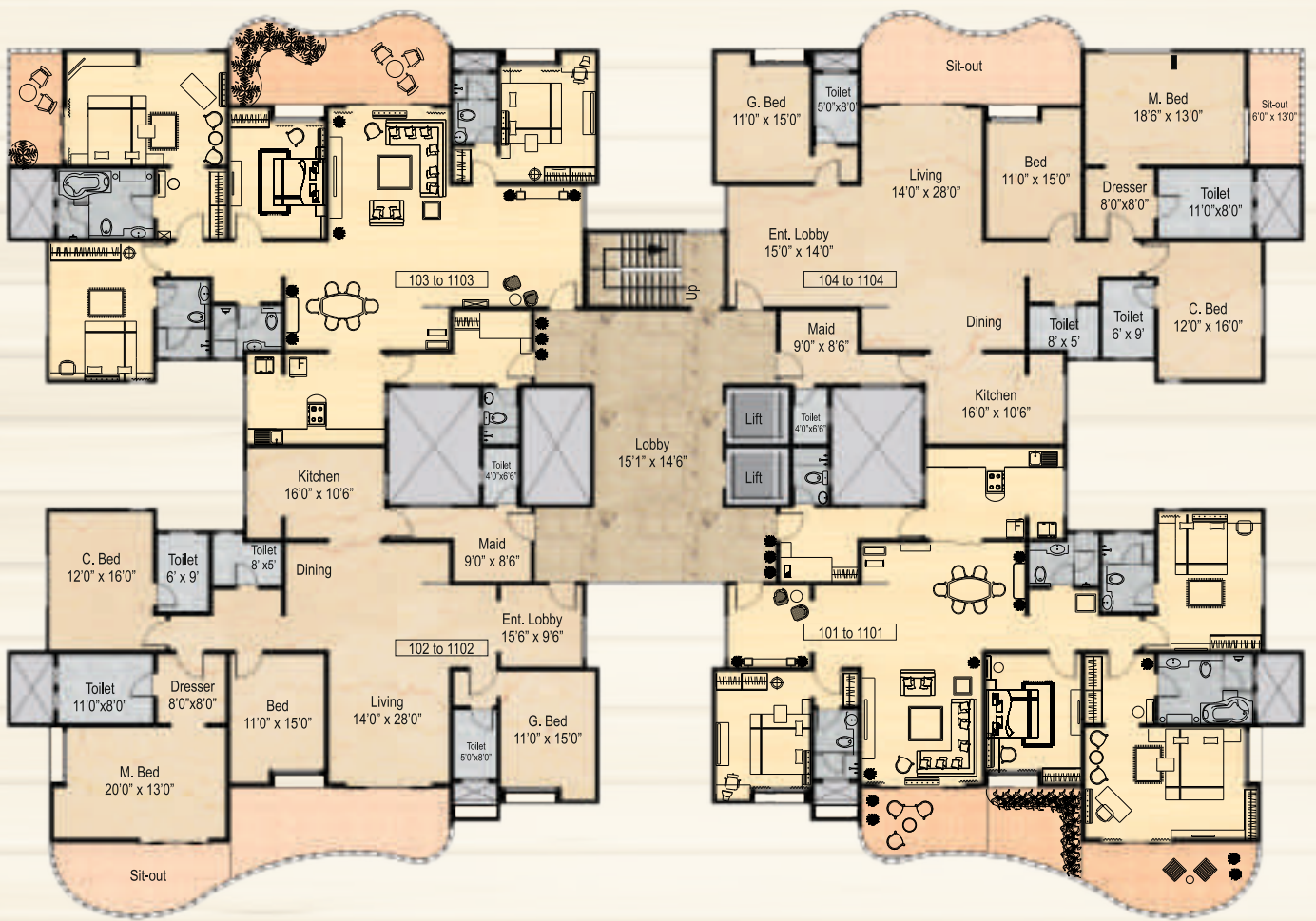
Typical Floor Plan - B Type (Clarinet)
